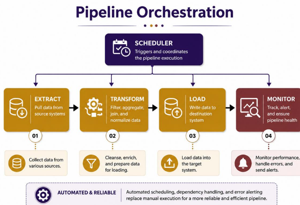
Figure 9.1. Pipeline Orchestration.
